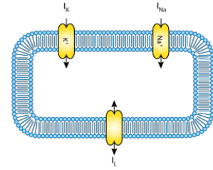
Figure 27. A schematic cell diagram describing the current flows across the cell bilipid membrane that are captured in the Hodgkin-Huxley model. The membrane ion channels are a sodium ( \text{Na}^+ ) channel, a potassium ( \text{K}^+ ) channel, and a leakage (L) channel (for chloride and other ions) through which the currents i_{Na} , i_K and i_L flow, respectively.
